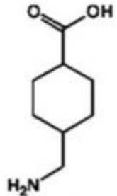
Structure of tranexamic acid
